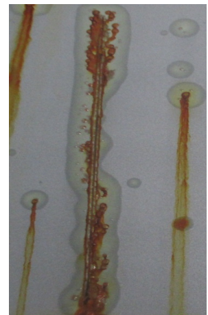
After 720 hours Salt Spray Test
