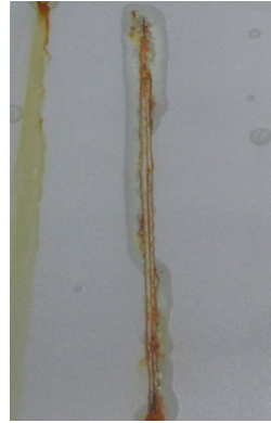
After 624 hours Salt Spray Test
