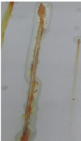
After 480 hours Salt Spray Test
